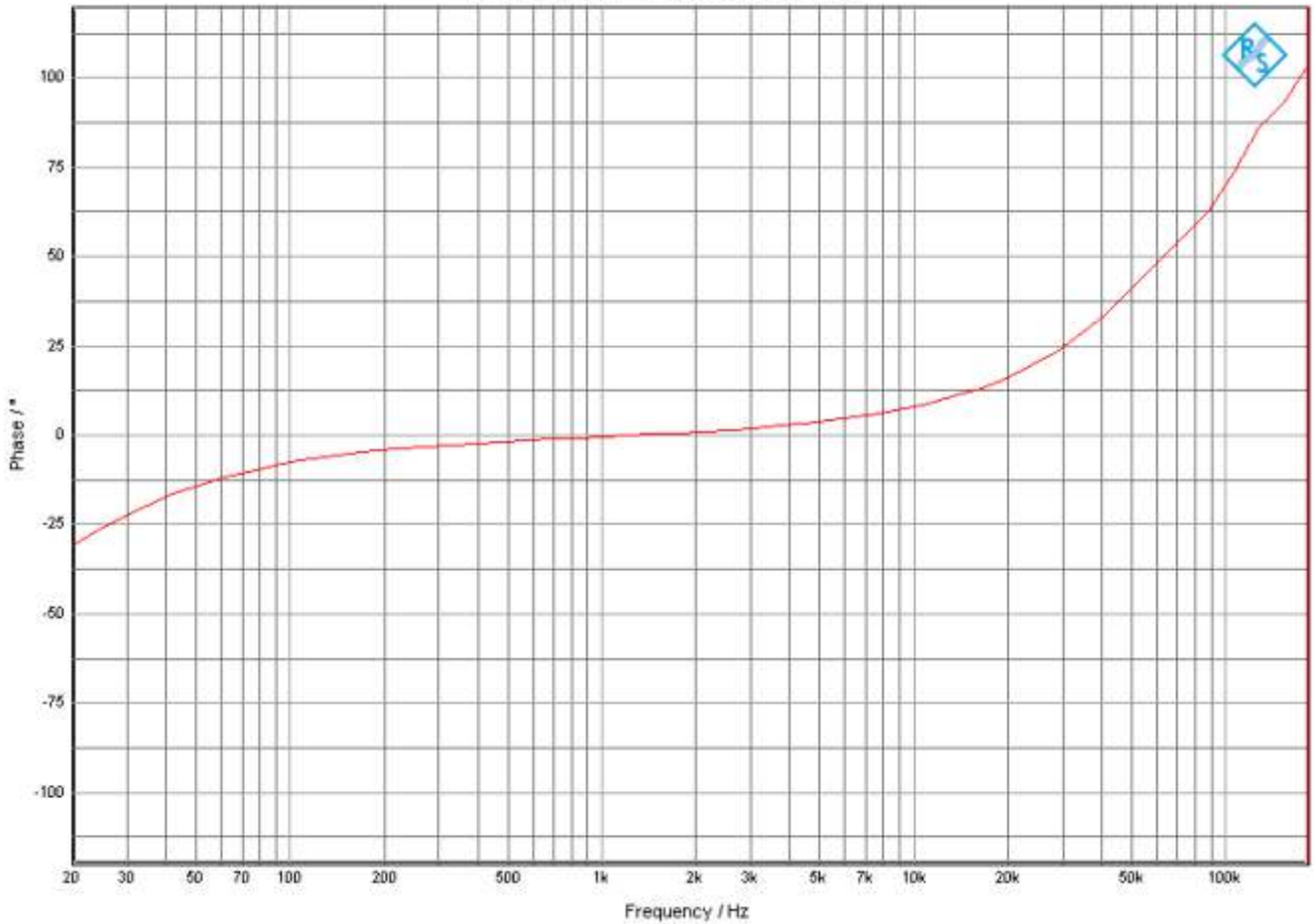
12SE3K3H - Phase response
