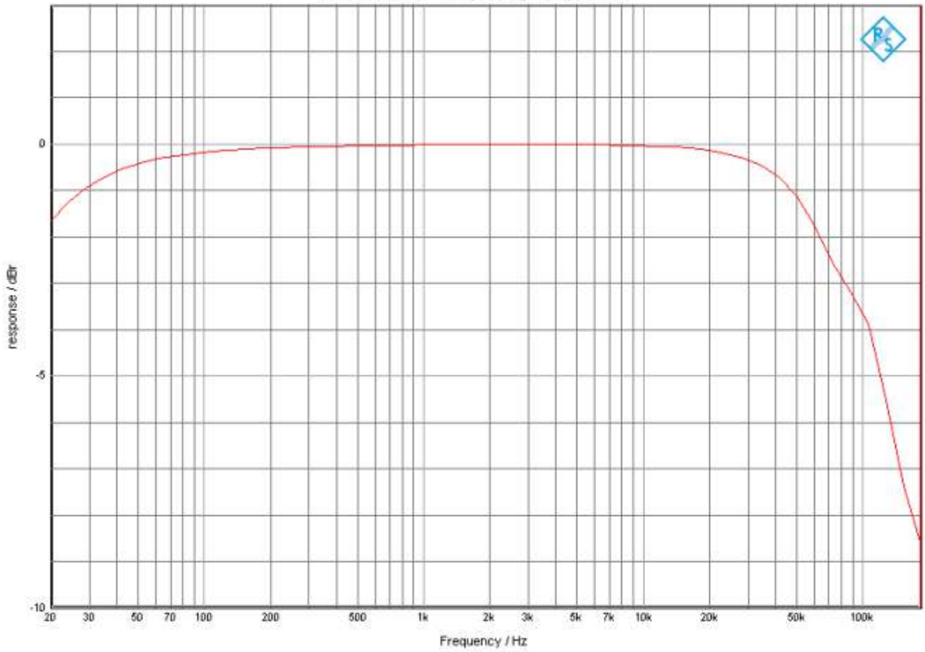
12SE3K3H - frequency response
